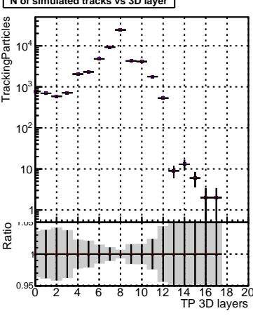
N of simulated tracks vs 3D layer
