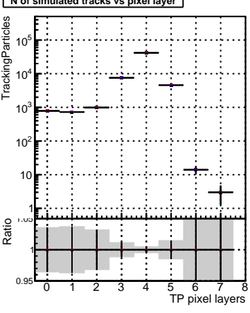
N of simulated tracks vs pixel layer
