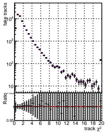
N of associated (recoToSim) fake tracks vs. \chi^2 for various methods: DGM, ttbar, PU, mkFit, Siter, updatedPR111, update, fixPropagation
