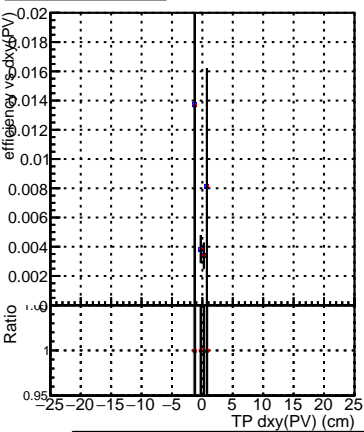
Efficiency vs Dxy(PV) - Legend DQM_ttbarPU_mkFit_5iter DQM_ttbarPU_mkFit_5iter_updatedPR111_update DQM_ttbarPU_mkFit_5iter_updatedPR111_update_fixPropagation
