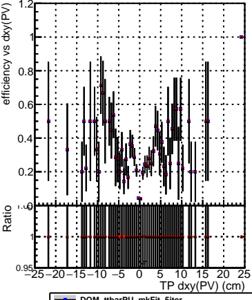
Efficiency vs Dxy(PV) DQM_ttbarPU_mkFit_5iter DQM_ttbarPU_mkFit_5iter_updatedPR111_update DQM_ttbarPU_mkFit_5iter_updatedPR111_update_fixPropagation
