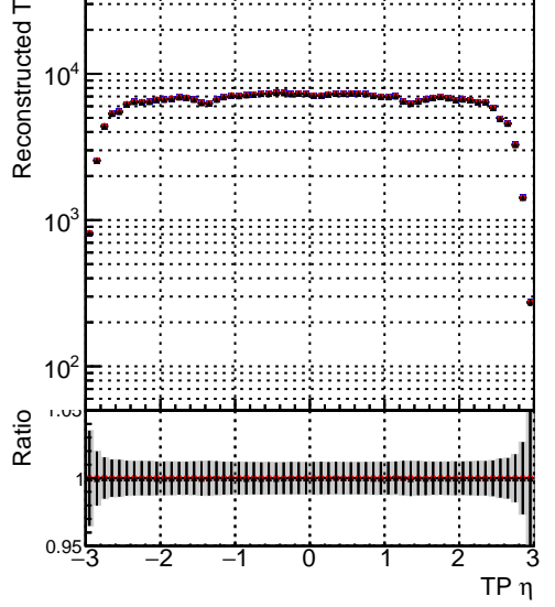
N of associated tracks (simToReco) vs TP η
