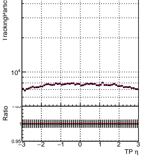
N of simulated tracks vs TP η
