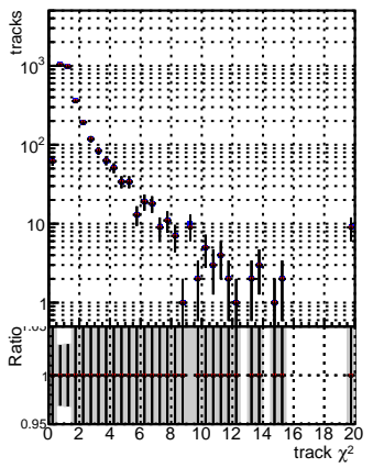
N of reco track vs. \chi^2 for different methods: BGM, ttbar, PU, mkFit, Siter, updatedPR11, update, fixPropagation.
