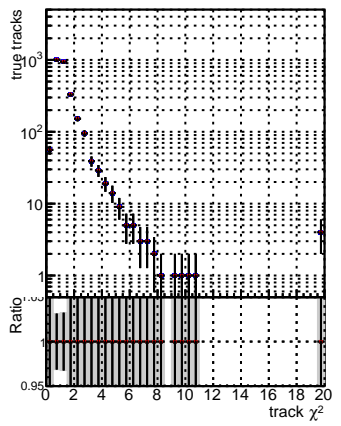
N of reco track vs. \chi^2 for different methods: BGM, ttbar, PU, mkFit, Siter, updatedPR11, update, fixPropagation.
