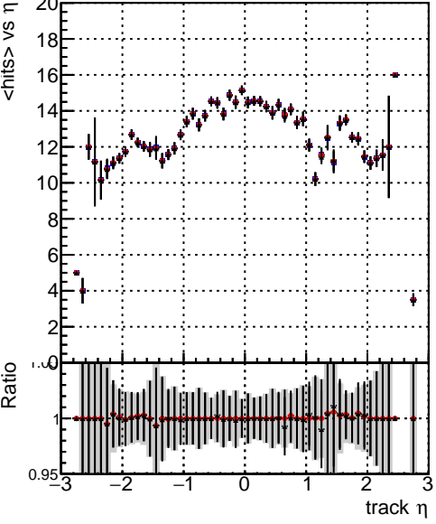
mean hits — DQM_ttbarPU_mkFit_5iter — DQM_ttbarPU_mkFit_5iter_updatedPR111_update — DQM_ttbarPU_mkFit_5iter_updatedPR111_update_fixPropagation
