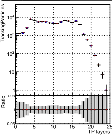
—■ DQM_mkFit_TTbarPU50_extractedGeoms_rescaleError100 —● DQM_mkFit_TTbarPU50_extractedGeoms_rescaleError100_pTCutOverlap0 —▲ DQM_mkFit_TTbarPU50_extractedGeoms_rescaleError100_pTCutOverlap0_dynamicChi2CutOverlap
