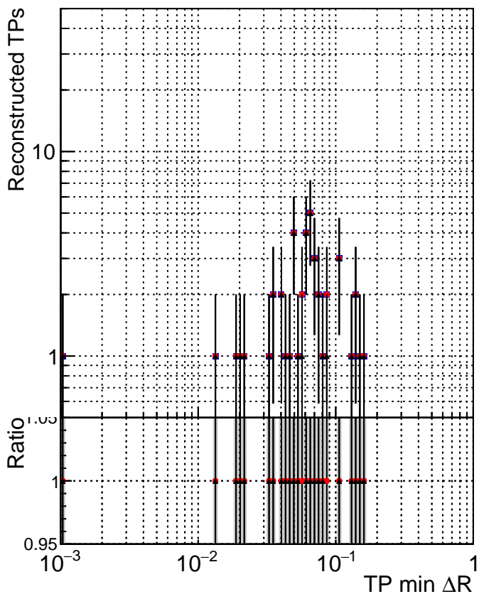
N of associated tracks (simToReco) vs ΔR(TP, jet)
