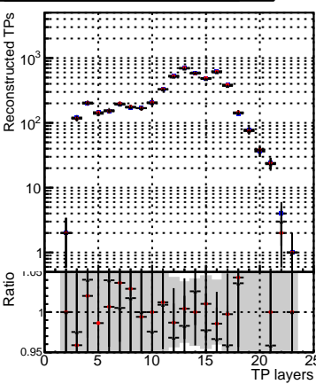
—● DQM_mkFit_TTbarPU50_extractedGeoms_rescaleError100 —● DQM_mkFit_TTbarPU50_extractedGeoms_rescaleError100_pTCutOverlap0p0 —● DQM_mkFit_TTbarPU50_extractedGeoms_rescaleError100_pTCutOverlap0p0_dynamicChi2CutOverlap
