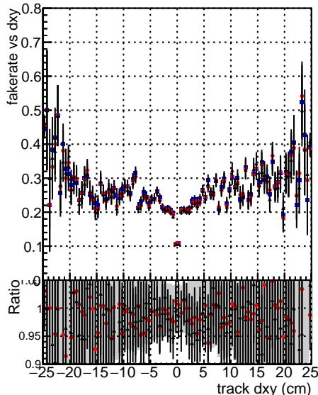
■ BGM mkFit ● TTbar PU50 extracted ● Geoms rescale ● Error100 ■ BGM mkFit ● TTbar PU50 extracted ● Geoms rescale ● Error100 ● pTCutOverlap0p0 ● dynamicChi2CutOverlap
