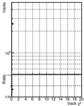
N of reco track vs. \chi^2 N of associated (recoToSim) tracks vs. \chi^2 N of associated (recoToSim) fake tracks vs. \chi^2 N of associated (recoToSim) looper tracks vs. \chi^2
