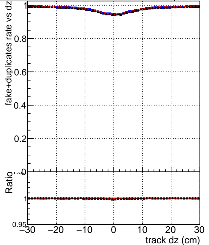
fake+duplicates vs dz —■— DQM_mkFit_TTbarPU50_extractedGeoms_rescaleError100 —●— DQM_mkFit_TTbarPU50_extractedGeoms_rescaleError100_pTCutOverlap0p0 —▲— DQM_mkFit_TTbarPU50_extractedGeoms_rescaleError100_pTCutOverlap0p0_dynamicChi2CutOverlap
