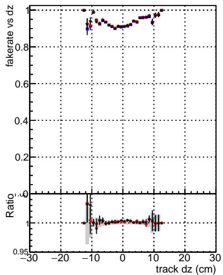
—●— DGM_mkFit_TTbar_PU50_extractedGeoms_rescaleError100 —●— DGM_mkFit_TTbar_PU50_extractedGeoms_rescaleError100 —●— DGM_mkFit_TTbar_PU50_extractedGeoms_rescaleError100 —●— BTCutOverlap0p0 —●— BTCutOverlap0p0 —●— BTCutOverlap0p0 —●— dynamicChi2CutOverlap —●— dynamicChi2CutOverlap —●— dynamicChi2CutOverlap
