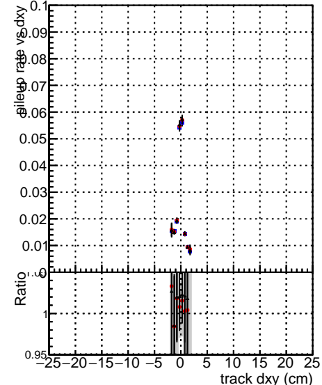
—●— DGM_mkFit_TTbar_PU50_extractedGeoms_rescaleError100 —●— DGM_mkFit_TTbar_PU50_extractedGeoms_rescaleError100_pTCutOverlap0p0 —●— DGM_mkFit_TTbar_PU50_extractedGeoms_rescaleError100_dynamicChi2CutOverlap
