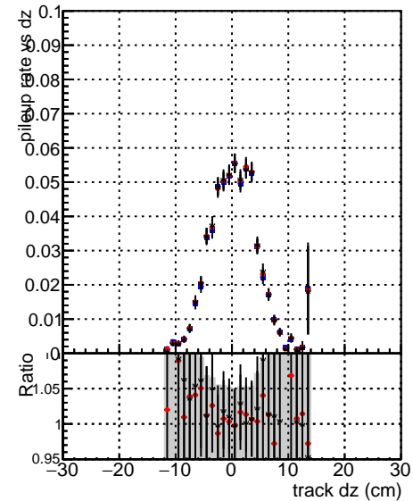
—●— DGM_mkFit_TTbar_PU50_extractedGeoms_rescaleError100 —●— DGM_mkFit_TTbar_PU50_extractedGeoms_rescaleError100_pTCutOverlap0p0 —●— DGM_mkFit_TTbar_PU50_extractedGeoms_rescaleError100_dynamicChi2CutOverlap
