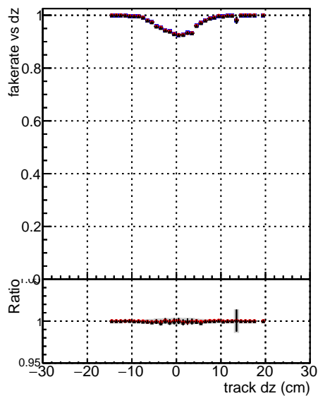
—●— DGM_mkFit_TTbar_PU50_extractedGeoms_rescaleError100 —●— DGM_mkFit_TTbar_PU50_extractedGeoms_rescaleError100_pTCutOverlap0p0 —●— DGM_mkFit_TTbar_PU50_extractedGeoms_rescaleError100_dynamicChi2CutOverlap
