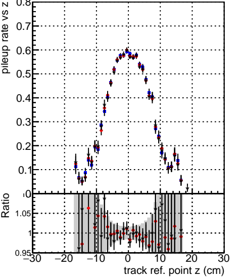
—●— DQM_mkFit_TTbarPU50_extractedGeoms_rescaleError100 —●— DQM_mkFit_TTbarPU50_extractedGeoms_rescaleError100_pTCutOverlap0p0 —●— DQM_mkFit_TTbarPU50_extractedGeoms_rescaleError100_dynamicChi2CutOverlap
