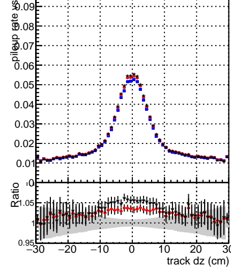
Pileup rate vs d dz
