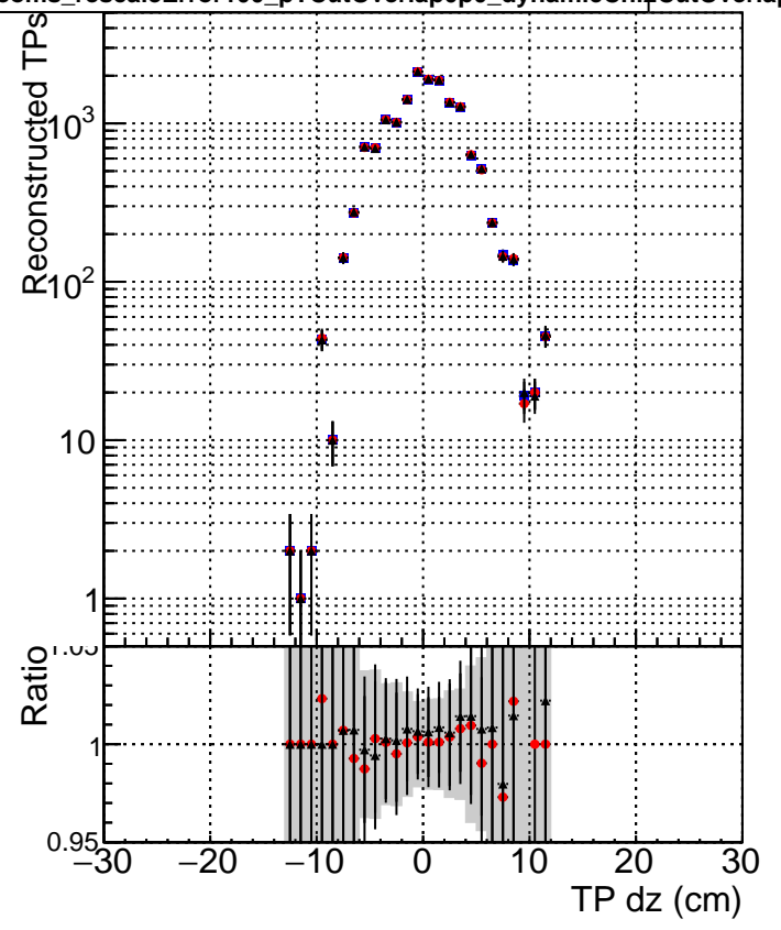
Legend: - DQM_mkFit_TTbarPU50_extractedGeoms_rescaleError100 (blue square) - DQM_mkFit_TTbarPU50_extractedGeoms_rescaleError100_pTCutOverlap0p0 (red circle) - DQM_mkFit_TTbarPU50_extractedGeoms_rescaleError100_pTCutOverlap0p0_dynamicChi2CutOverlap (black triangle)
