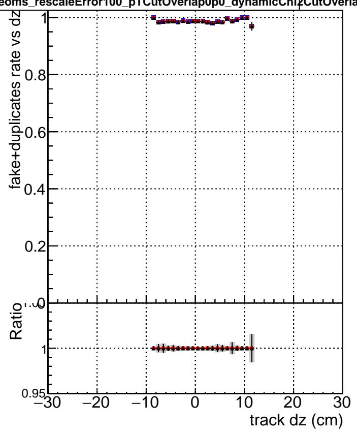
Legend: -■- DQM_mkFit_TTbarPU50_extractedGeoms_rescaleError100 -●- DQM_mkFit_TTbarPU50_extractedGeoms_rescaleError100_pTCutOverlap0p0 -▲- DQM_mkFit_TTbarPU50_extractedGeoms_rescaleError100_pTCutOverlap0p0_dynamicChi2CutOverlap
