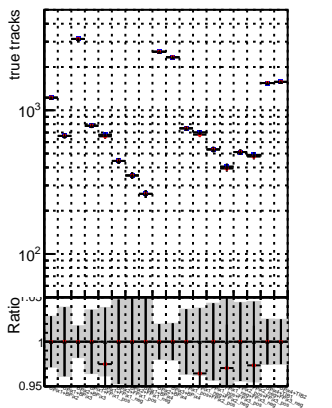
N of reco track vs. N of associated (recoToSim) tracks vs normalized \chi^2 N of associated (recoToSim) looper tracks vs normalized \chi^2
