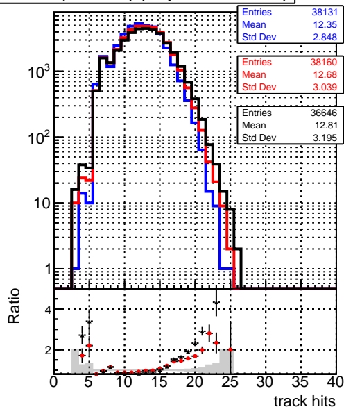
mean hit — DQM_mkFit_TTbarPU50_extractedGeoms_rescaleError100_pTCutOverlap0p0 — DQM_mkFit_TTbarPU50_extractedGeoms_rescaleError100_pTCutOverlap0p0 — DQM_mkFit_TTbarPU50_extractedGeoms_rescaleError100_pTCutOverlap0p0_dynamicChi2CutOverlap
