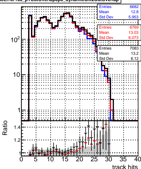
mean hit DQM_mkFit_TTbarPU50_extractedGeoms_rescaleError100 DQM_mkFit_TTbarPU50_extractedGeoms_rescaleError100_pTCutOverlap0p0 DQM_mkFit_TTbarPU50_extractedGeoms_rescaleError100_pTCutOverlap0p0_dynamicChi2CutOverlap
