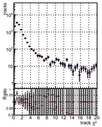
N of reco track vs. \chi^2 DGM mFit TTbar PU50 extractedGeoms rescaleError100 pTCutOverlap0p0 dynamicChi2CutOverlap overSet
