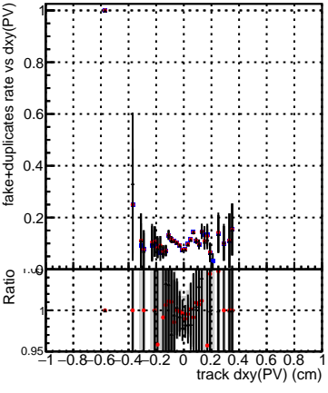
Efficiency —●— DQM_mkFit_TTbarPU50_extractedGeoms_rescaleError100 —●— DQM_mkFit_TTbarPU50_extractedGeoms_rescaleError100_pTCutOverlap0p0 fake+duplicates —●— DQM_mkFit_TTbarPU50_extractedGeoms_rescaleError100_pTCutOverlap0p0_dynamicChi2CutOverlap
