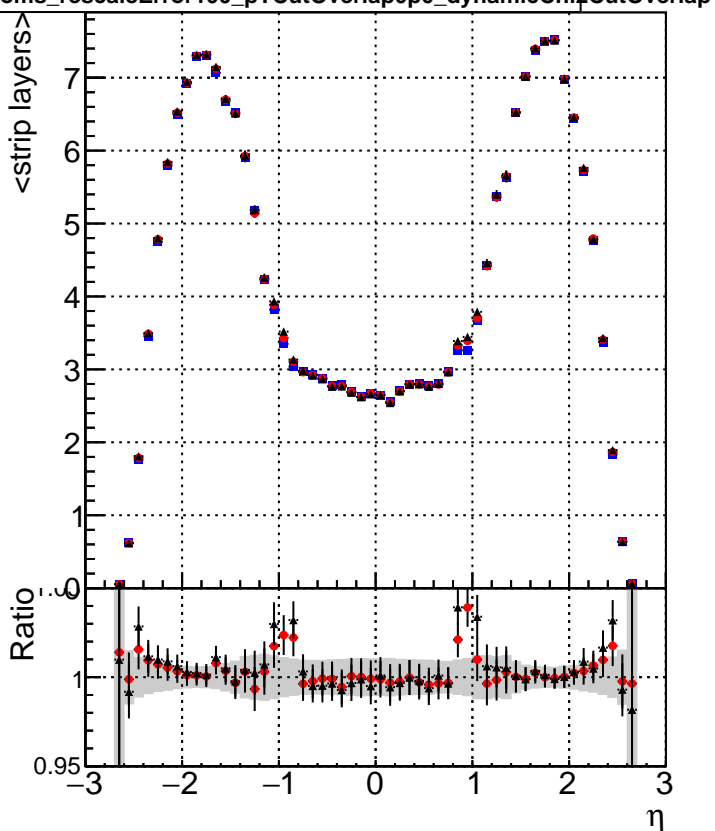
Legend for STRIP hits plots: ■ DQM_mkFit_TTbarPU50_extractedGeoms_rescaleError100 ● DQM_mkFit_TTbarPU50_extractedGeoms_rescaleError100_pTCutOverlap0p0 ▲ DQM_mkFit_TTbarPU50_extractedGeoms_rescaleError100_pTCutOverlap0p0_dynamicChi2CutOverlap
