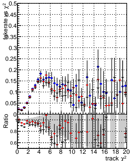
◆ DGM_mkFit_TTbar_PU50_extracted_Geoms_rescale_Error100 ■ DGM_mkFit_TTbar_PU50_extracted_Geoms_rescale_Error100_pTCutOverlap0p0_dynamicChi2CutOverlap
