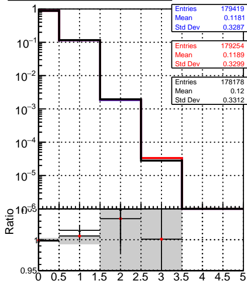
mean hit DQM_mkFit_TTbarPU50_extractedGeoms_rescaleError100 DQM_mkFit_TTbarPU50_extractedGeoms_rescaleError100_pTCutOverlap0p0 DQM_mkFit_TTbarPU50_extractedGeoms_rescaleError100_pTCutOverlap0p0_dynamicChi2CutOverlap
