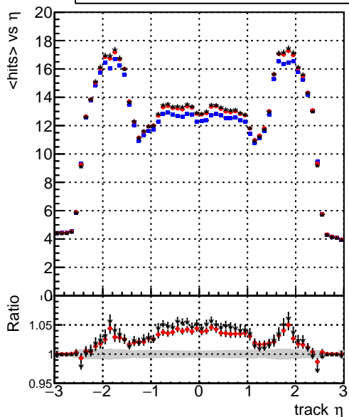
mean hit DQM_mkFit_TTbarPU50_extractedGeoms_rescaleError100 DQM_mkFit_TTbarPU50_extractedGeoms_rescaleError100_pTCutOverlap0p0 DQM_mkFit_TTbarPU50_extractedGeoms_rescaleError100_pTCutOverlap0p0_dynamicChi2CutOverlap
