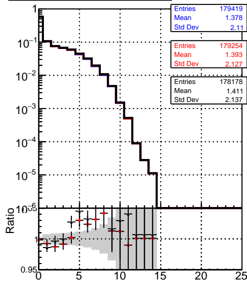
mean hit DQM_mkFit_TTbarPU50_extractedGeoms_rescaleError100 DQM_mkFit_TTbarPU50_extractedGeoms_rescaleError100_pTCutOverlap0p0 DQM_mkFit_TTbarPU50_extractedGeoms_rescaleError100_pTCutOverlap0p0_dynamicChi2CutOverlap
