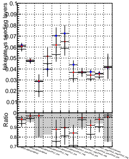
Fake rate vs. —•— DGM_mkFit —•— TTbar_PU50_extracted —•— Geoms_rescale —•— Error100 —•— DGM_mkFit —•— TTbar_PU50_extracted —•— Geoms_rescale —•— Error100 —•— pTCutOverlap0p0 —•— dynamicChi2CutOverlap
