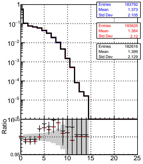
mean hit — DQM_mkFit_TTbarPU50_extractedGeoms_rescaleError100 — DQM_mkFit_TTbarPU50_extractedGeoms_rescaleError100_pTCutOverlap0p0 — DQM_mkFit_TTbarPU50_extractedGeoms_rescaleError100_pTCutOverlap0p0_dynamicChi2CutOverlap
