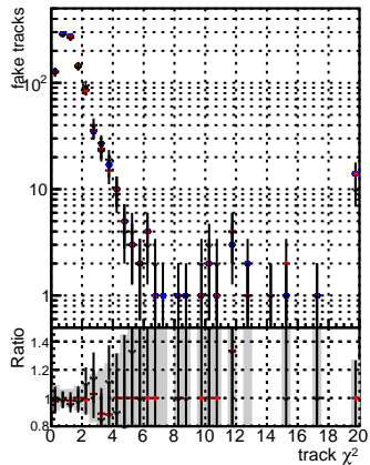
N of associated (recoSim) looper tracks vs normalized \chi^2
