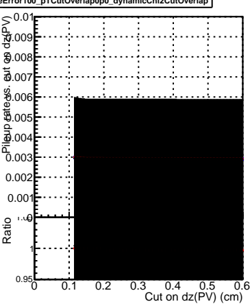
DQM_mkFit_TTbarPU50_extractedGeoms_rescaleError100_pTCutOverlap0p0_dynamicChi2CutOverlap
