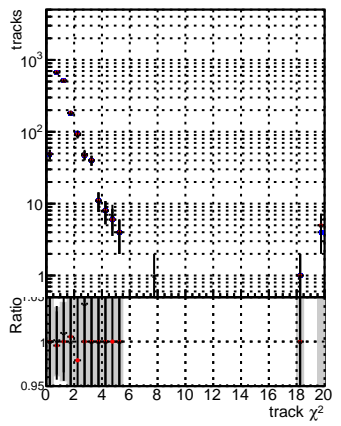
N of reco track vs. \chi^2 for various methods: DGM mkFit, TTbarPU50, extractedGeoms, rescale, Error100, DTCutOverlap0p0, dynamicChi2CutOverlap
