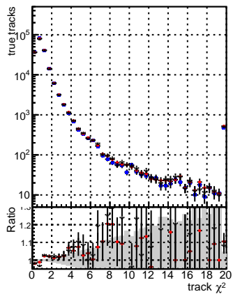
N of associated (recoSim) tracks vs normalized \chi^2
