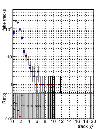
N of reco track vs. \chi^2 for various methods: DGM (blue circles), mFit (red squares), TbarPU50 (grey triangles), extractedGeoms (black diamonds), rescaleError100 (black squares), pTCutOverlap0p0 (black circles), dynamicChi2CutOverlap (black circles).
