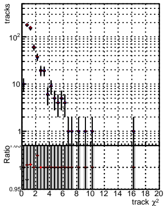
N of reco track vs. \chi^2 for various methods: DGM, mKFIT, Tbar, PU50, extractedGeoms, rescale, Error100, pTCutOverlap0p0, dynamicChi2CutOverlap
