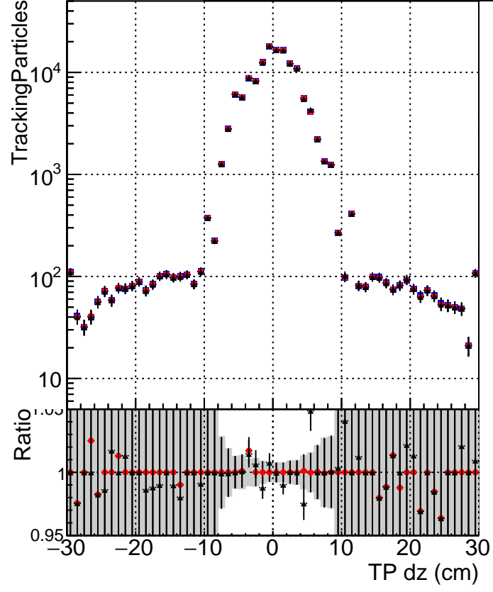
N of simulated tracks vs TP dz (cm) ■ DQM_mkFit_TTbarPU50_extractedGeoms_rescaleError100 ● DQM_mkFit_TTbarPU50_extractedGeoms_rescaleError100_pTCutOverlap0p0 ▲ DQM_mkFit_TTbarPU50_extractedGeoms_rescaleError100_pTCutOverlap0p0_dynamicChi2CutOverlap
