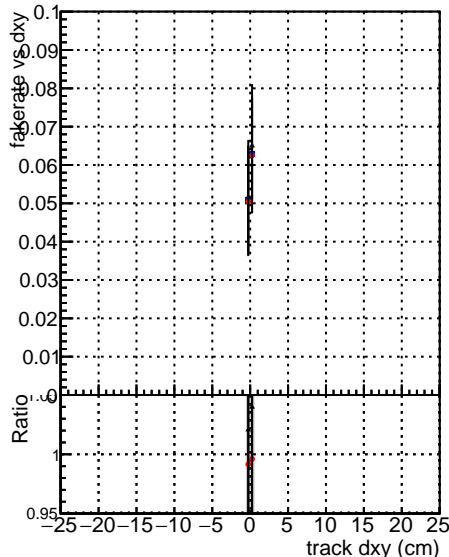
DGM_mkFit_TTbar_PU50_extracted_Geoms_rescale_Error100 DGM_mkFit_TTbar_PU50_extracted_Geoms_rescale_Error100_pTCutOverlap0p0 DGM_mkFit_TTbar_PU50_extracted_Geoms_rescale_Error100_pTCutOverlap0p0_dynamicChi2CutOverlap
