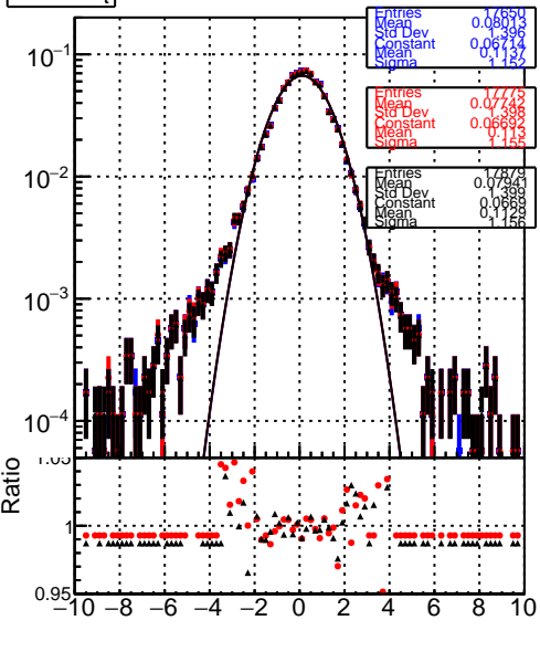
pull of p_t
