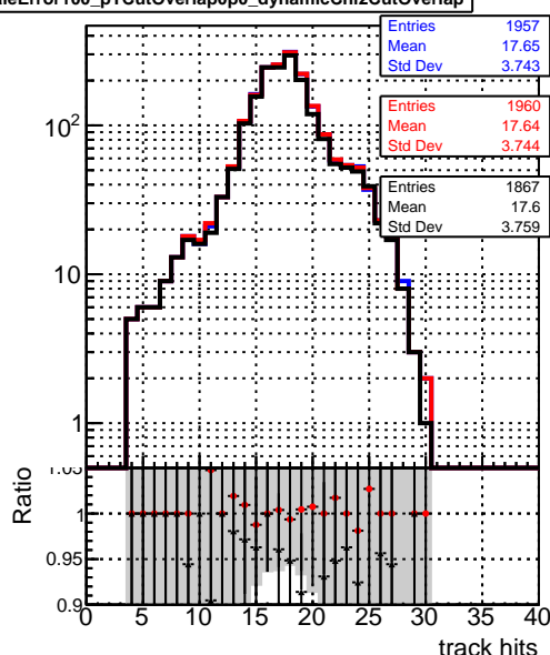
track hits
