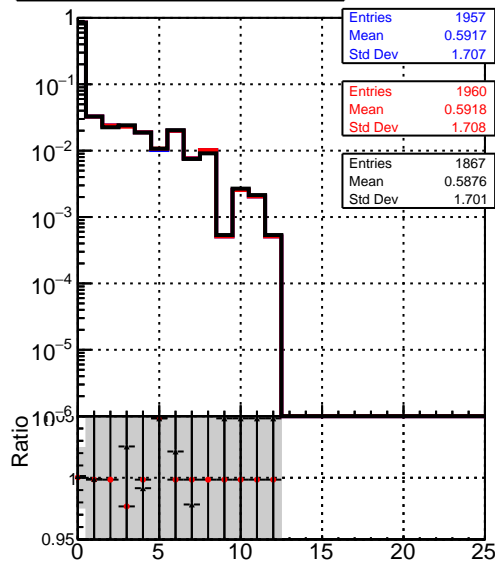
track hits
