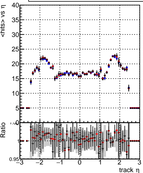
mean hit \eta — DQM_mkFit_TTbarPU50_extractedGeoms_rescaleError100 — DQM_mkFit_TTbarPU50_extractedGeoms_rescaleError100_pTCutOverlap0p0 — DQM_mkFit_TTbarPU50_extractedGeoms_rescaleError100_pTCutOverlap0p0_dynamicChi2CutOverlap
