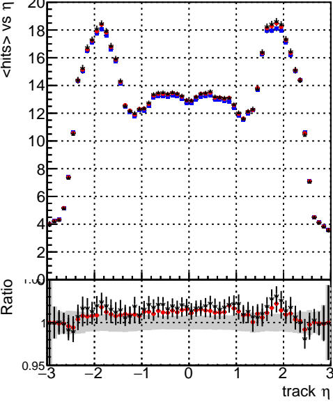
mean hit — DQM_mkFit_TTbarPU50_extractedGeoms_rescaleError100 — DQM_mkFit_TTbarPU50_extractedGeoms_rescaleError100_pTCutOverlap0p0 — DQM_mkFit_TTbarPU50_extractedGeoms_rescaleError100_pTCutOverlap0p0_dynamicChi2CutOverlap
