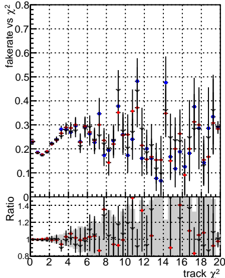
◆ BQM_mkFit ◆ TTbar_PU50_extracted ◆ Geoms_rescale ◆ Error100 ◆ BQM_mkFit ◆ TTbar_PU50_extracted ◆ Geoms_rescale ◆ Error100 ◆ pTCutOverlap0p0 ◆ dynamicChi2CutOverlap
