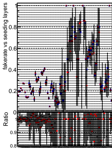
◆ BQM_mkFit ◆ TTbar_PU50_extracted ◆ Geoms_rescale ◆ Error100 ◆ BQM_mkFit ◆ TTbar_PU50_extracted ◆ Geoms_rescale ◆ Error100 ◆ pTCutOverlap0p0 ◆ dynamicChi2CutOverlap
