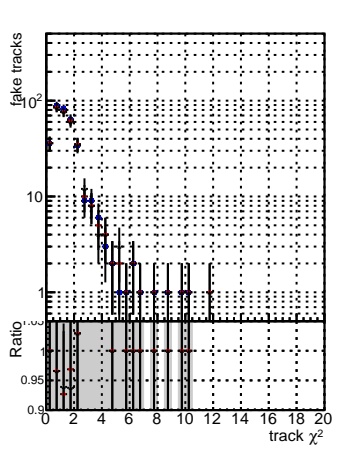
N of reco track vs. \chi^2 for various methods: DGM, mKF, T-bar, PU50, extractedGeoms, rescale, Error100, pTCutOverlap0p0, dynamicChi2CutOverlap
