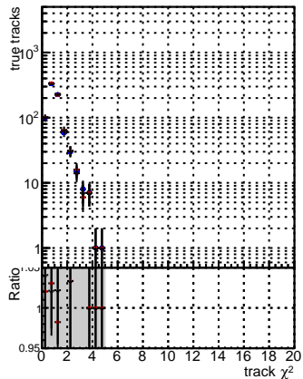
N of reco track vs. DGM mFit \bar{P} 50 extractedGeoms rescaleError100 DGM mFit \bar{P} 50 extractedGeoms rescaleError100 pTCutOverlap0p0 DGM mFit \bar{P} 50 extractedGeoms rescaleError100 pTCutOverlap0p0 dynamicChi2CutOverlap
