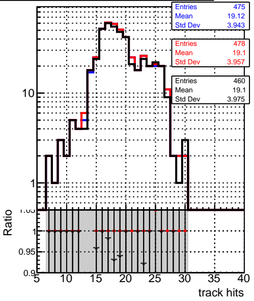
mean hit
