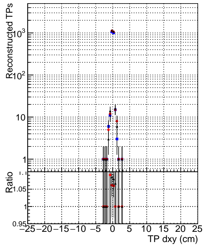
Legend: - Blue square: DQM_mkFit_TTbarPU50_extractedGeoms_rescaleError100 - Red circle: DQM_mkFit_TTbarPU50_extractedGeoms_rescaleError100_pTCutOverlap0p0 - Black triangle: DQM_mkFit_TTbarPU50_extractedGeoms_rescaleError100_pTCutOverlap0p0_dynamicChi2CutOverlap
