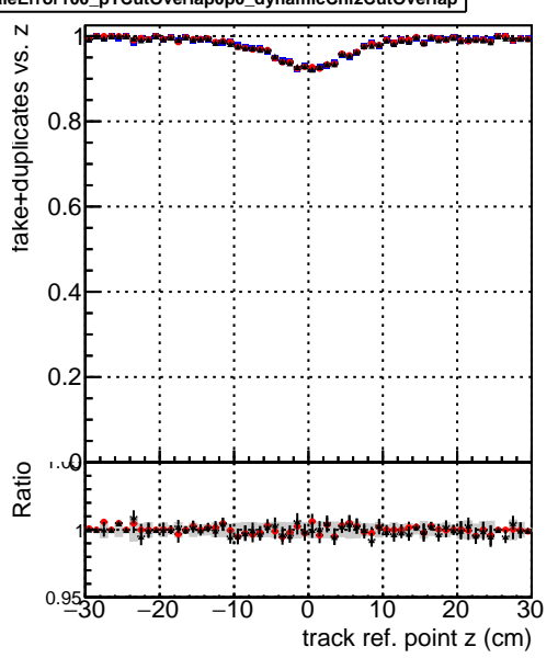
fake+duplicates vs. z — DQM_mkFit_TTbarPU50_extractedGeoms_rescaleError100 — DQM_mkFit_TTbarPU50_extractedGeoms_rescaleError100_pTCutOverlap0p0 — DQM_mkFit_TTbarPU50_extractedGeoms_rescaleError100_pTCutOverlap0p0_dynamicChi2CutOverlap
