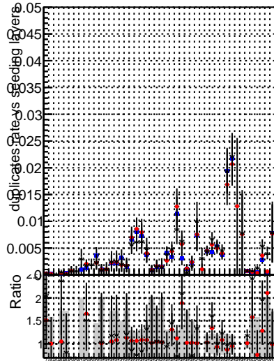
BGM mkFit TTbar PU50 extracted Geoms rescale Error100 BGM mkFit TTbar PU50 extracted Geoms rescale Error100 pTCutOverlap0p0 dynamicChi2CutOverlap
