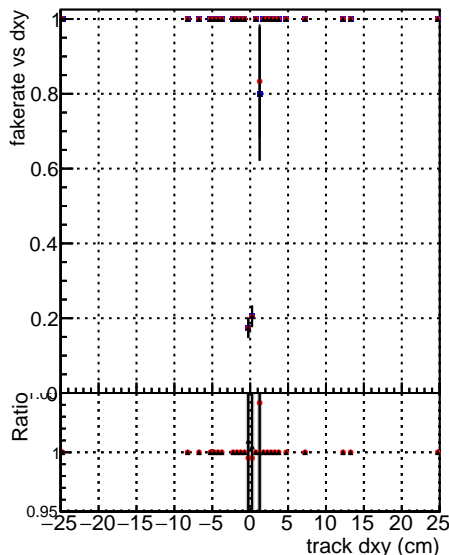
—●— DGM_mkFit_TTbar_PU50_extracted_Geoms_rescale_Error100 —●— DGM_mkFit_TTbar_PU50_extracted_Geoms_rescale_Error100_dTCutOverlap0p0_dynamicChi2CutOverlap
