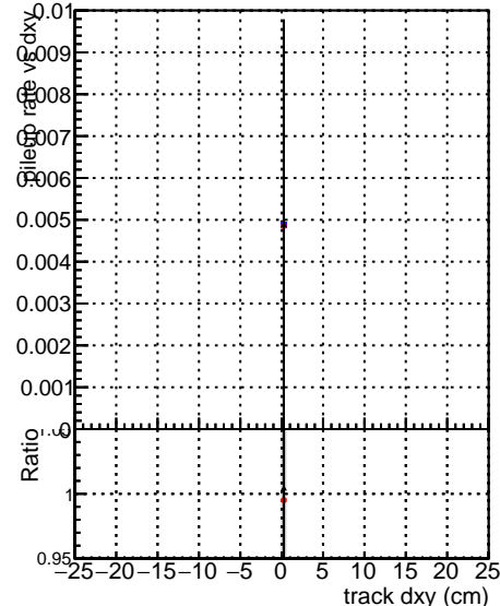
—●— DGM_mkFit_TTbar_PU50_extracted_Geoms_rescale_Error100 —●— DGM_mkFit_TTbar_PU50_extracted_Geoms_rescale_Error100_dTCutOverlap0p0_dynamicChi2CutOverlap
