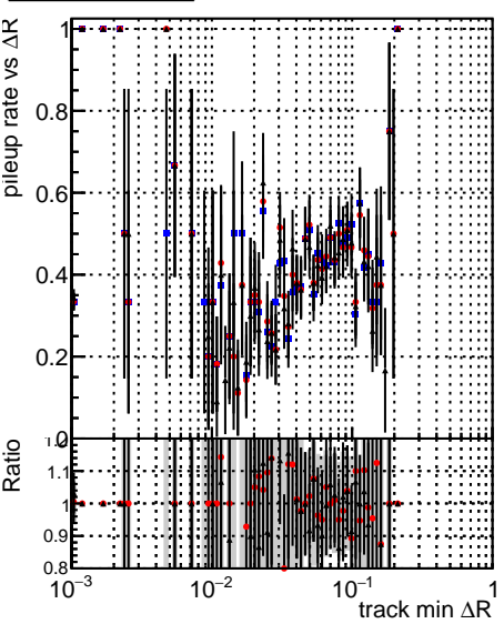
—●— DQM_mkFit_TTbarPU50_extractedGeoms_rescaleError100 —●— DQM_mkFit_TTbarPU50_extractedGeoms_rescaleError100_pTCutOverlap0p0 —●— DQM_mkFit_TTbarPU50_extractedGeoms_rescaleError100_pTCutOverlap0p0_dynamicChi2CutOverlap
